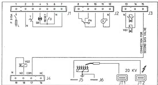
TYPE MM32
