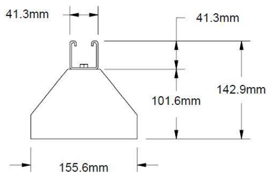
SUPPORT DE CLIM FOOTBLOC 600 (Charge maxi 300kg)
