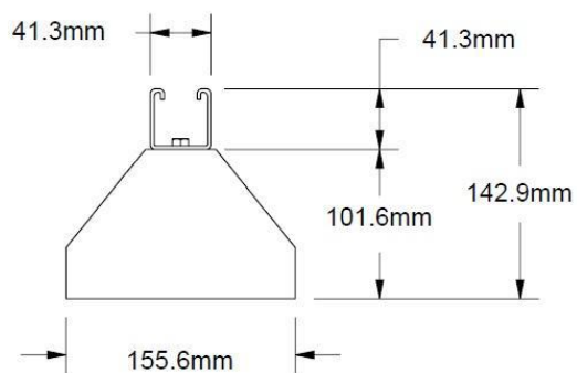
SUPPORT DE CLIM FOOTBLOC 400 (Charge maxi 300kg)
