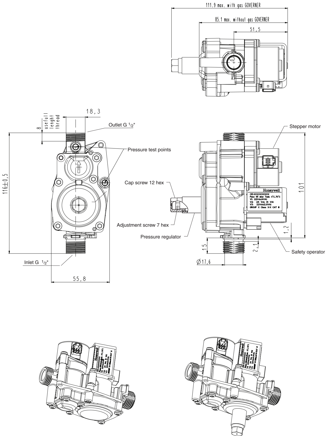
Fig. 1. Dimensional drawing
